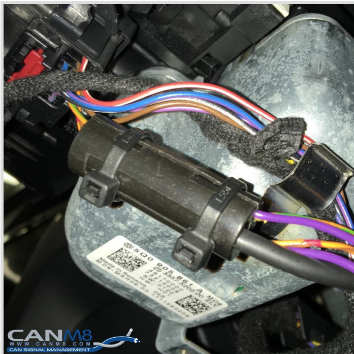
CAN Wiring at the steering column (Contactless Reader installed)
