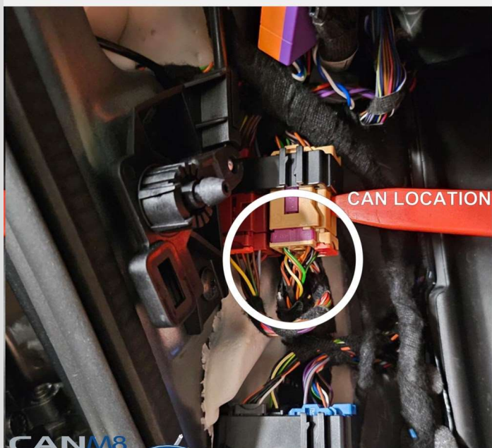
Brown connector behind the driver side kick panel
