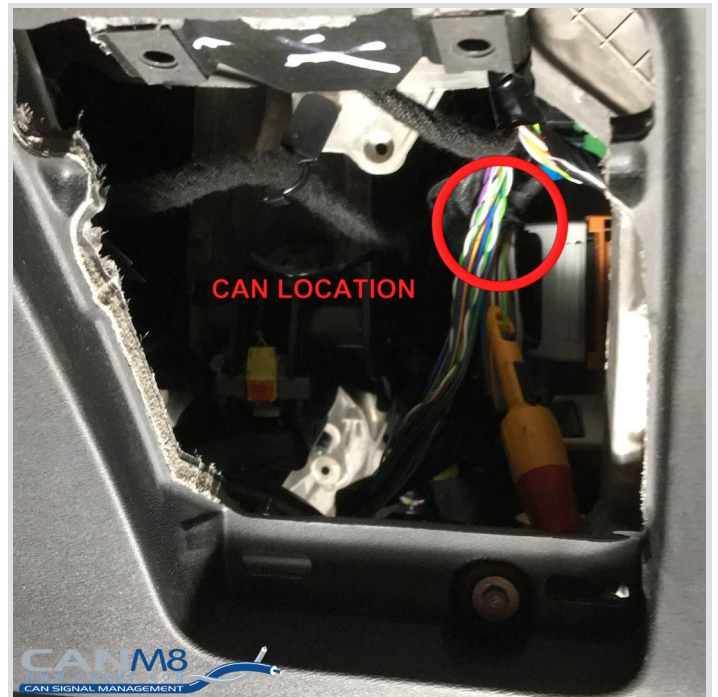
Access to the CEM behind the dash pocket
