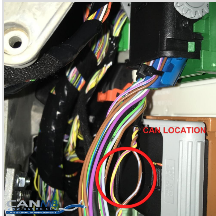
CAN wiring
